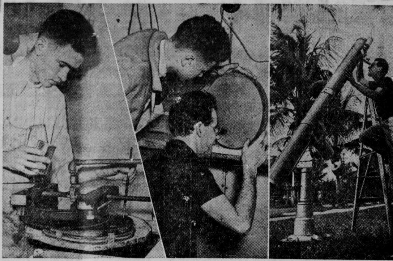
Two Miami, Fla., youths, Lynn C. Burkhart and Arthur P. Smith Jr., are operating a "factory" they built and equipped at a total cost of $20, and are turning out telescopes that have attracted the praise of Dr. G. H. Lutz, America's foremost telescopic engineer. Left: Smith applies carborundum to the grinding glass as the mirror rotates back and forth. Twelve inches in diameter, this mirror is very large for any but a professional attempt. Center: The mirror is studied for possible defects. It takes approximately eight months to grind the mirror. Right: Here's the finished product being inspected by Burkhart. It's ready for use in star studies.
