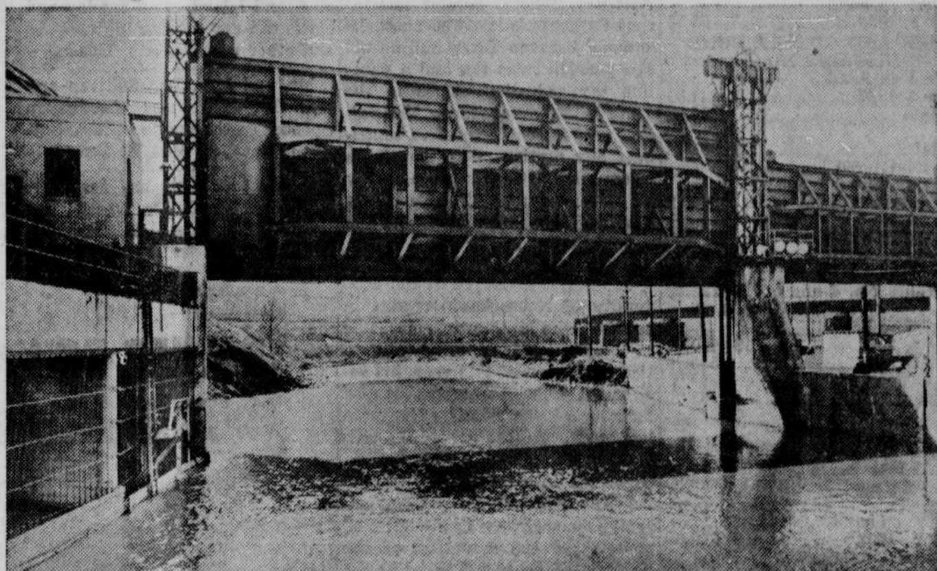
View of the massive steel gates installed by the Westinghouse Electric company near Pittsburgh, Pa., to prevent floods from entering and damaging the plants during the frequent high waters in the rivers converging in the Pittsburgh district. When lowered into place, these gates cause the water to back up behind them. The three giant pumps force the water through the intakes in lower left, where it is guided around the flood wall and out into Turtle creek, in the background, over a long spillway.
