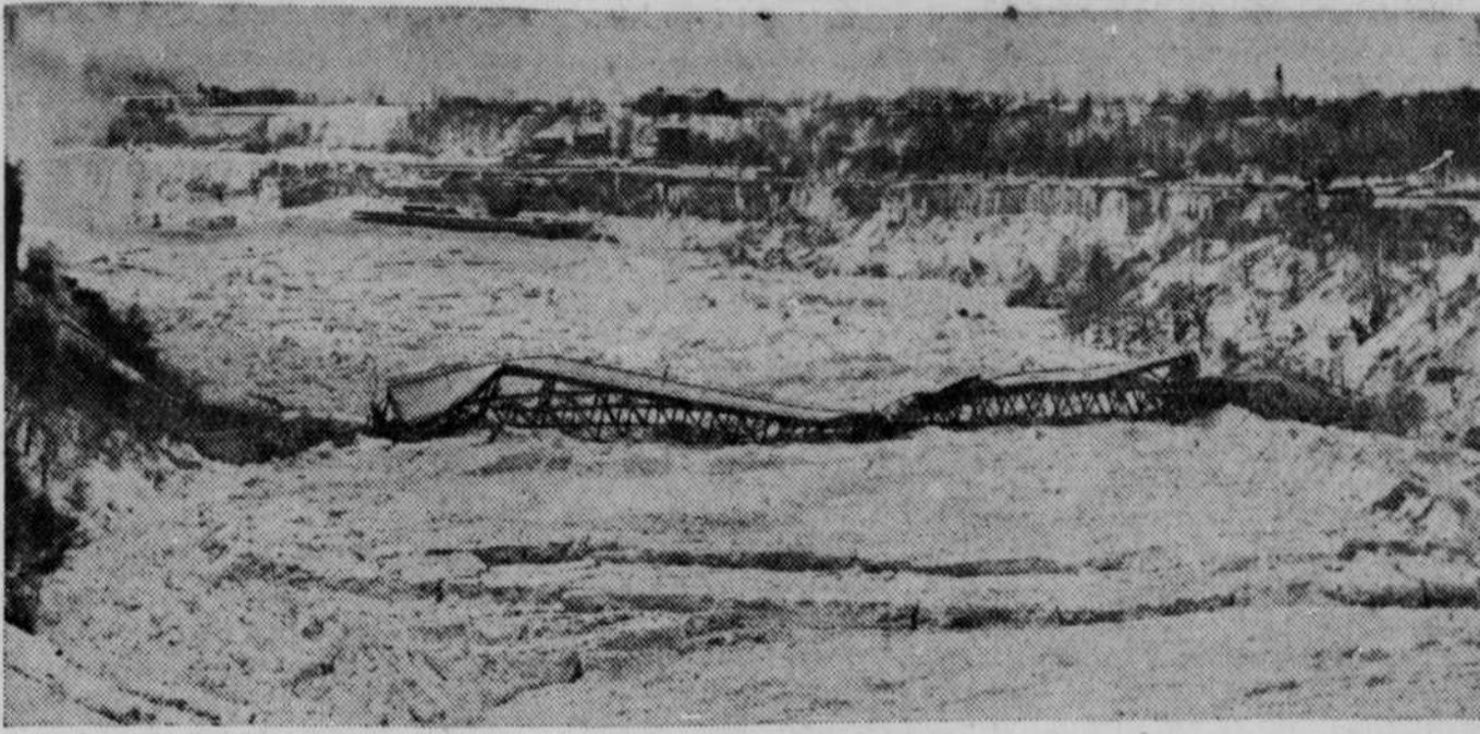
This twisted mass of steel girders among mountainous blocks of ice is all that remains of the 40-year-old Falls View International bridge which collapsed into the ice-filled gorge below Niagara falls after resisting an ice jam for 24 hours. This view of the collapsed "honeymoon bridge" was made from the American side. The noise of the crash of the 4,500,000-pound structure blotted out for a moment the roar of Niagara falls, 500 yards upstream. Thousands of spectators watched as the girders buckled. Workmen who had been sent into the gorge to strengthen the bridge's supports narrowly escaped death when the crash came.
