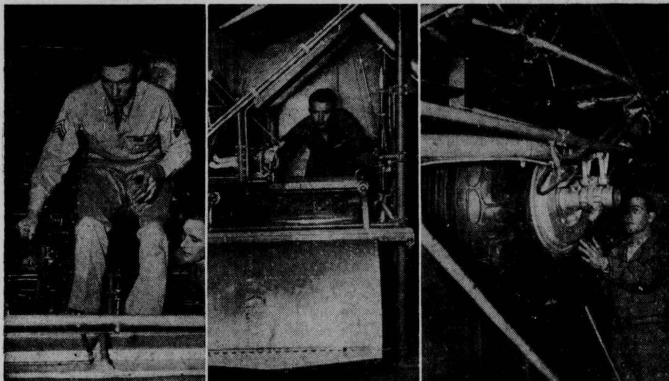
Today it is possible for almost any enlisted man to become a skilled mechanic or technician for Uncle Sam. These pictures, made at Chanute Field, Ill., show some of the phases of training to qualify as hydraulic experts. Left: A hydraulic "mock up." This is a B-18A pilot seat with all the controls which operate the hydraulic system of the plane. Center: One of the important functions of hydraulics in a bomber is the opening and closing of bomb bays. Here Pvt. Willis Nord checks the operations. Right: Those huge wheels used on the powerful planes are retracted by hydraulic power. Here a wheel is being lifted.
