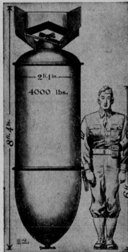
This is a photo-diagram of the dreaded 4,000 pound super-block-buster, made in the United States, and dropped on Germany in night and day raids by American fliers and RAF men. Approximately 2,200 pounds of the two-ton bomb are TNT and other secret explosives. The rest are shell and fuses. Dropped from a plane 20,000 feet up, the bomb strikes the ground at pulverizing 600-mile-an-hour speed.
