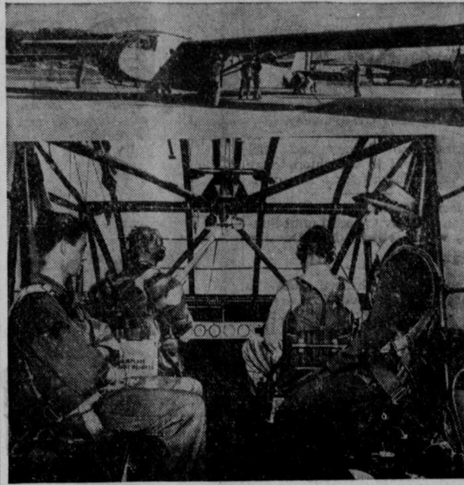
These pictures, just released by the army air forces, show the first of the new 15-place troop-carrying gliders, the CG-4A, now in quantity production. The glider can carry 15 fully equipped men, including pilot and co-pilot. It has a wing span of 83 feet, 8 inches, and a length of 48 feet, 3 inches. At the top we get a good idea of the glider's size by comparing it with the size of the men. Below is an interior view showing pilot and co-pilot at the controls.
