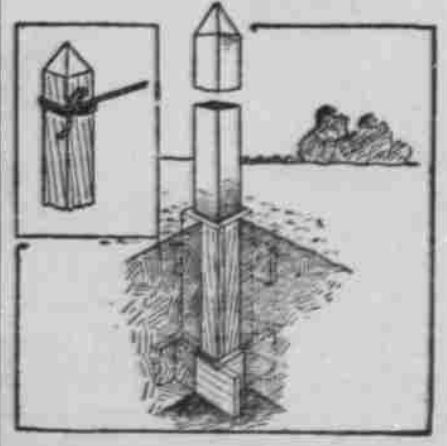
Removable Posts.
